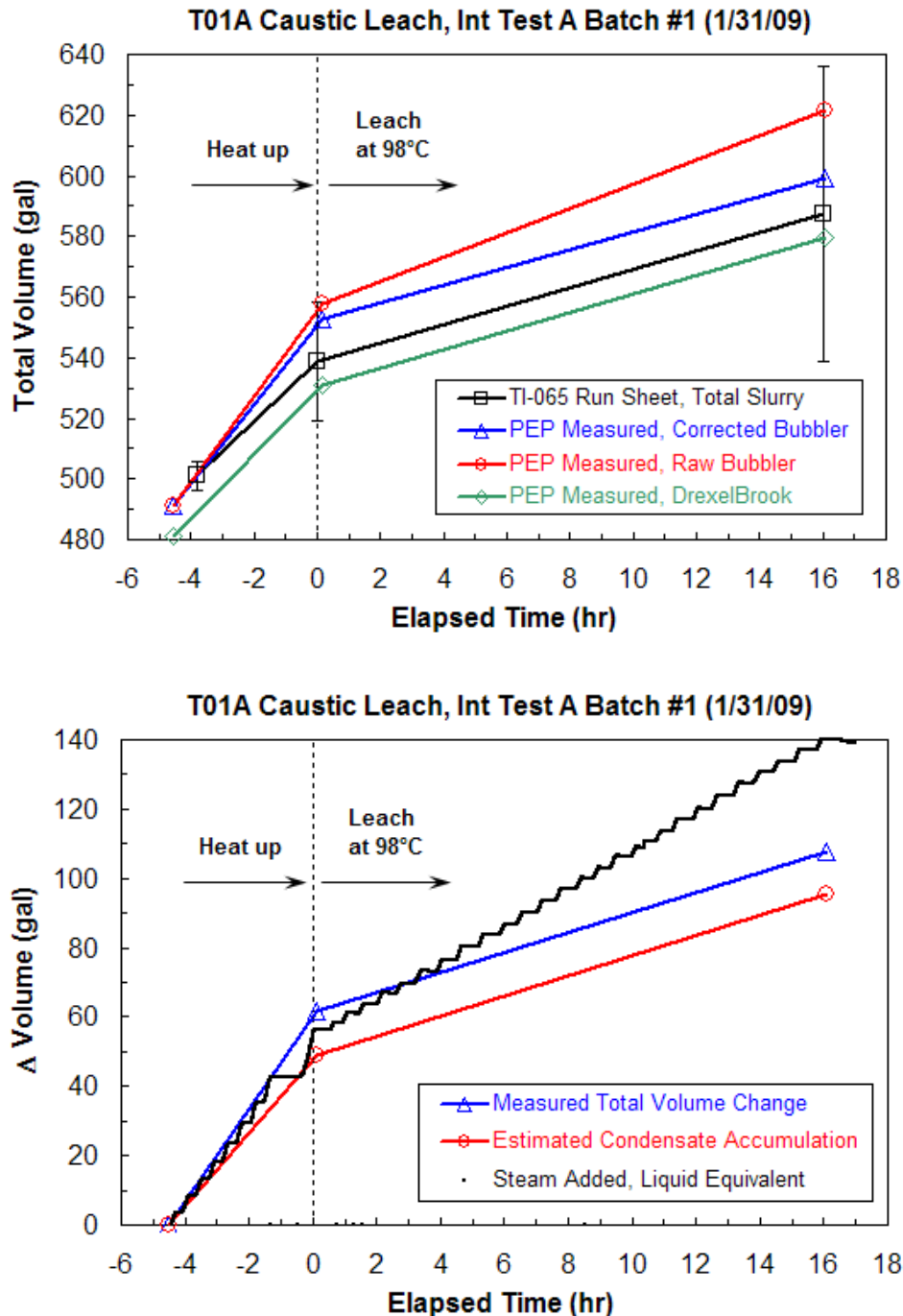
Figure 3.4. Volumes in UFP-T01A Associated with Direct Steam Injection During the Heat-Up and Caustic-Leach Periods of Integrated Test A Batch 1: Upper—Total Slurry-Condensate Mixture Volume as Determined from Multiple Level Sensors Compared to TI-065 Run Sheet Targets (with ranges shown); Lower—Slurry Component Volume Changes ( \Delta ) (e.g., the total increase in the slurry-condensate mixture volume and the estimated volume of condensate accumulated compared to the total amount of steam added [as an equivalent liquid volume at the vessel temperature])
