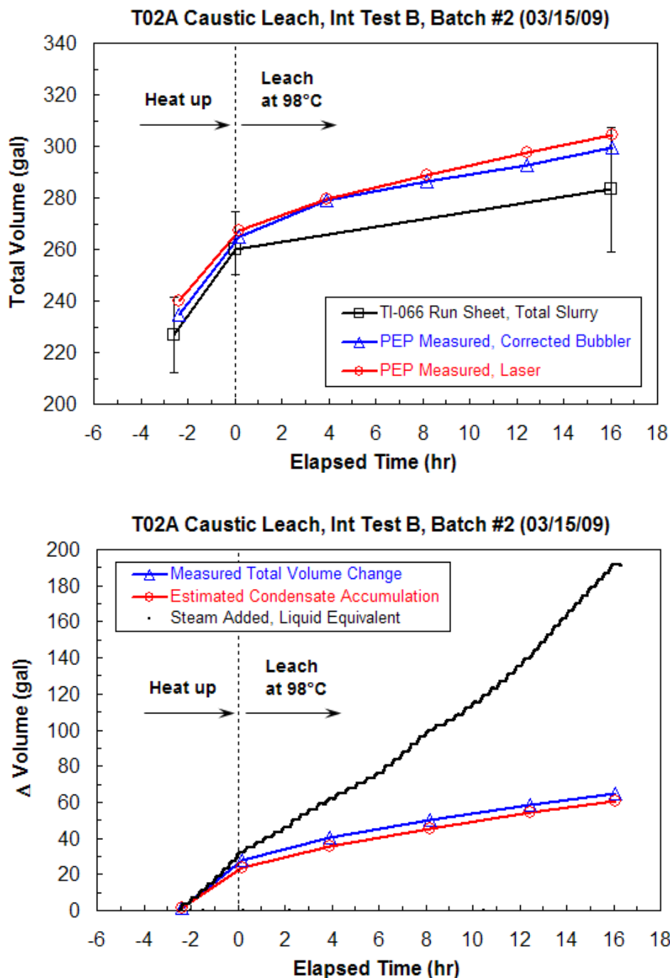
Figure 3.5. Volumes in UFP-T02A Associated with Direct Steam Injection During the Heat-Up and Caustic-Leach Periods of Integrated Test B Batch 2: Upper—Total Slurry-Condensate Mixture Volume as Determined from Two Level Sensors Compared to TI-066 Run Sheet Targets (with ranges shown); Lower—Slurry Component Volume Changes ( \Delta ) (e.g., the total increase in the slurry-condensate mixture volume and the estimated volume of condensate accumulated from laser data compared to the total amount of steam added [as an equivalent liquid volume at the vessel temperature])
