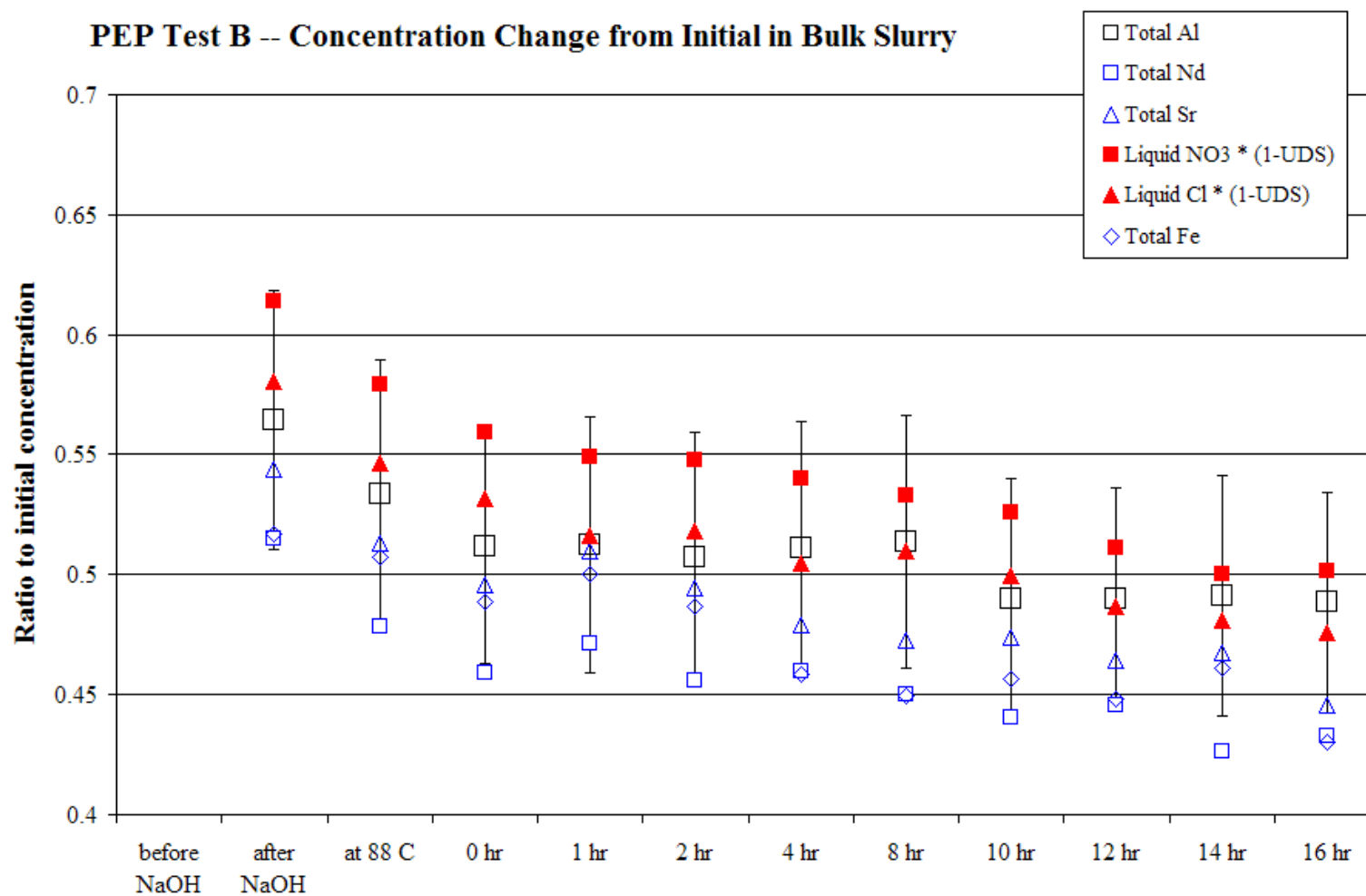
Figure 4.2. Dilution Factors with 95% Confidence Intervals During PEP Integrated Test B (caustic leaching in UFP-T02A)
