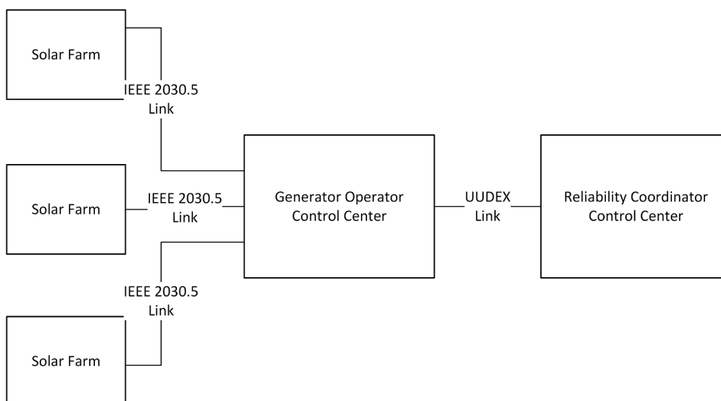
Figure 1.1: IEEE 2030.5 and UUDEX
