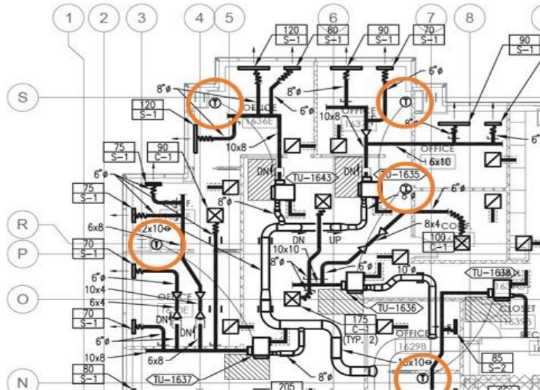
Figure 6018.1 Mechanical Floor Plan Showing Thermostats in Multiple Locations
