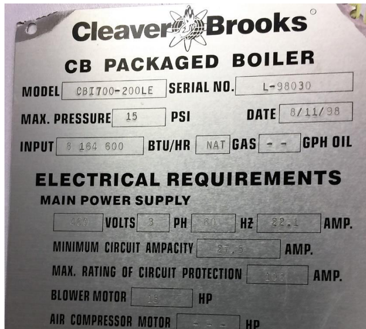
Figure 6005.7 Boiler Nameplate Data
