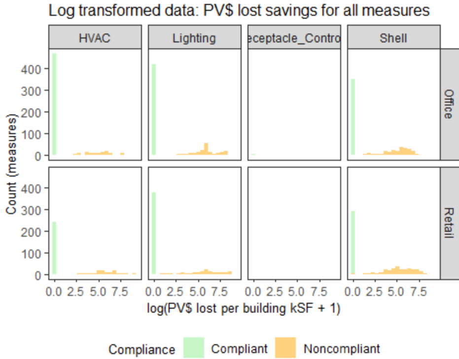
Figure 6.1. Log-Transformed Data: PV$ Lost Savings for All Measures
