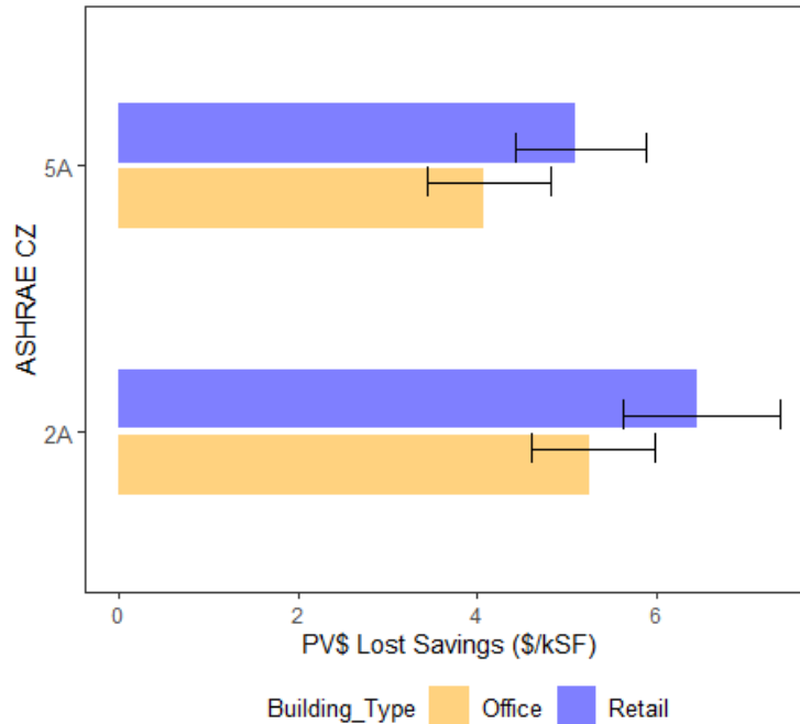
Figure 6.9. Estimated Mean PV$ Lost Savings by Building Type and ASHRAE CZ with 80% Confidence Intervals
