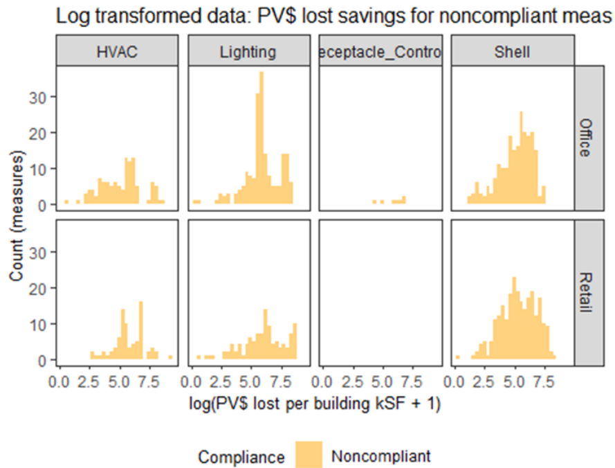
Figure 6.2. Log-Transformed Data: PV$ Lost Savings for Noncompliant Measures
