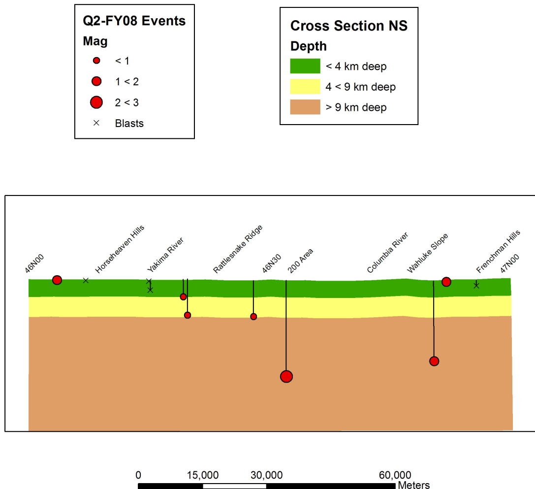
Figure 5.2. Cross-Sectional Depiction (along 119W30 longitude) of Earthquakes Occurring in the Hanford Monitoring Area between January 1, 2008 and March 31, 2008 (second quarter)
