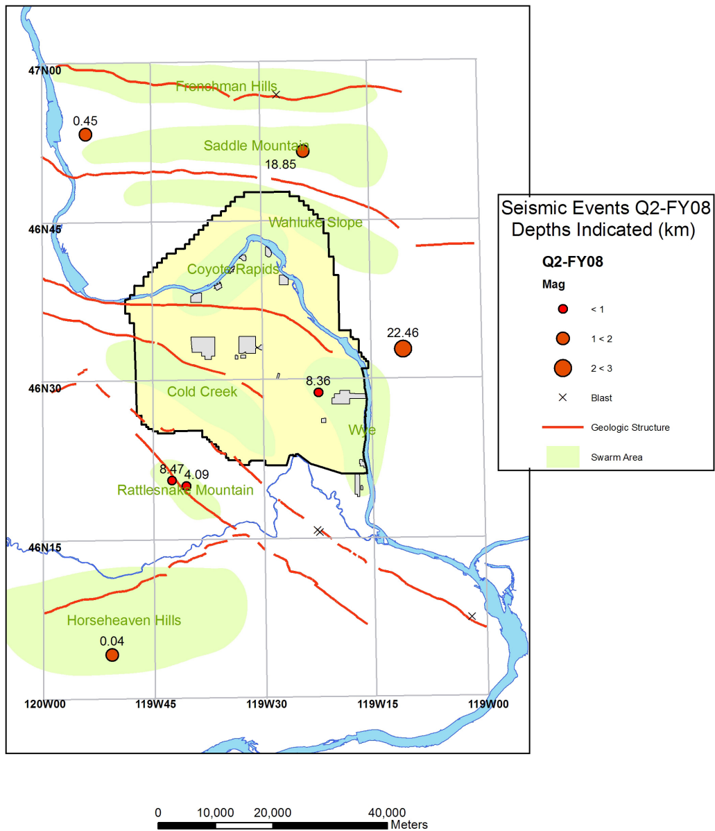
Figure 5.1. Earthquakes Occurring in the Hanford Monitoring Area Between January 1, 2008 and March 31, 2008 (second quarter)
