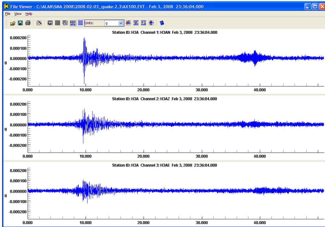
Figure 6.1. February 3, 2008 Microearthquake Acceleration Time Histories at 300 Area SMA
