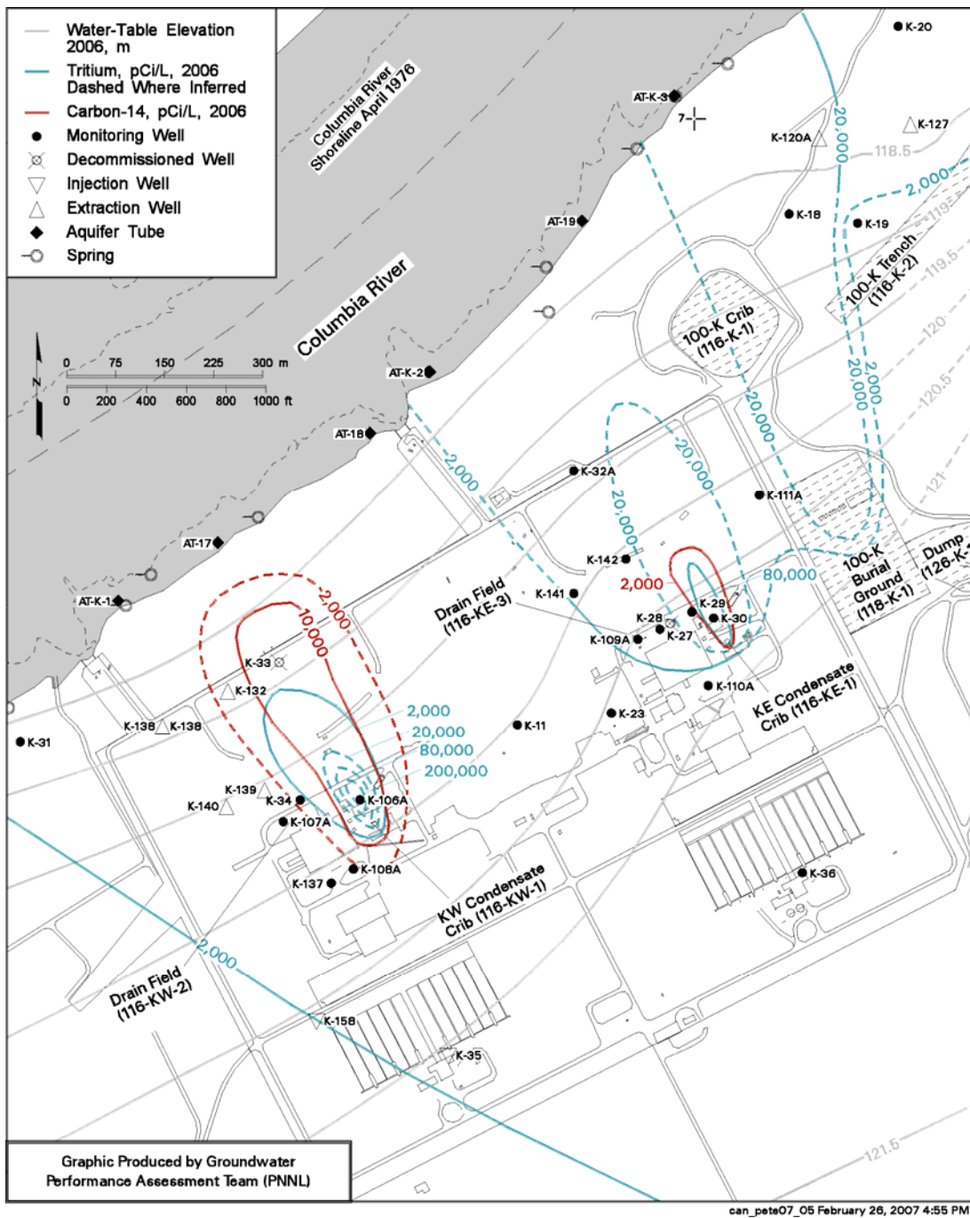
Figure 1. Location Map for Wells in the Vicinity of the K Basins, and 2006 Tritium and Carbon-14 Plumes (after PNNL-16346).
